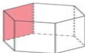
hexagonal prism
