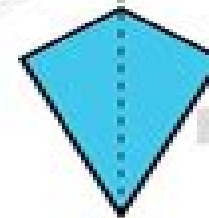
Kite 1 line of symmetry
