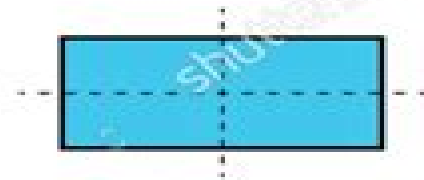
Rectangle 2 lines of symmetry
