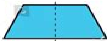
Isosceles Trapezoid 1 line of symmetry
