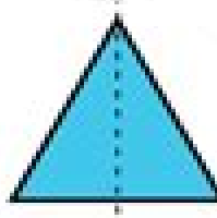
Isosceles Triangle 1 line of symmetry
