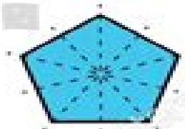
Regular Pentagon 5 lines of symmetry
