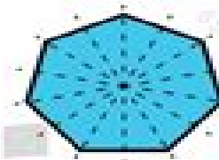
Regular Heptagon 7 lines of symmetry
