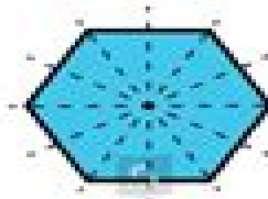
Regular Hexagon 6 lines of symmetry
