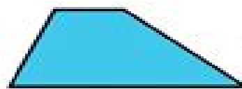
Trapezoid No lines of symmetry
