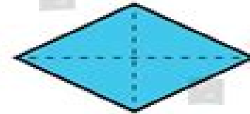
Rhombus 2 lines of symmetry
