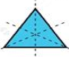
Equilateral Triangle 3 lines of symmetry
