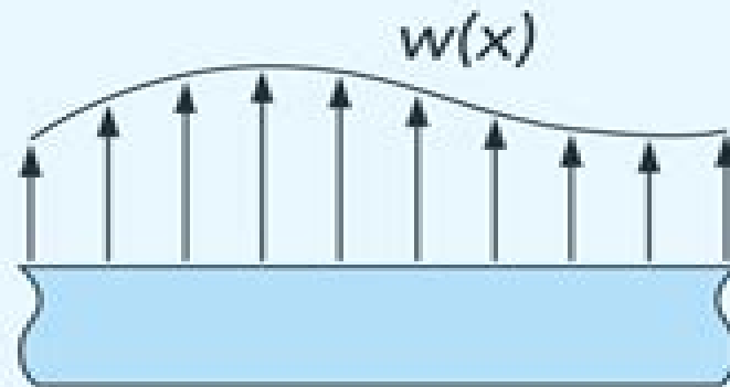
Positive external distributed load
