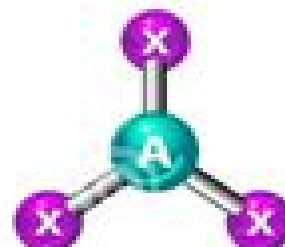
Trigonal planar
