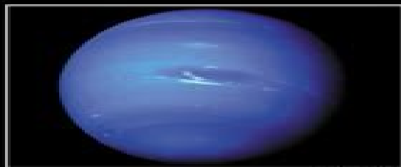
Neptune
