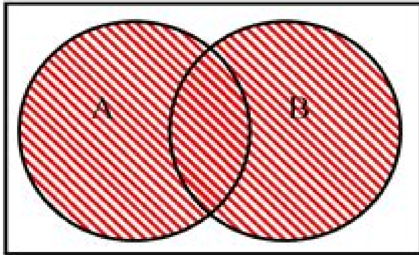
Set Union
