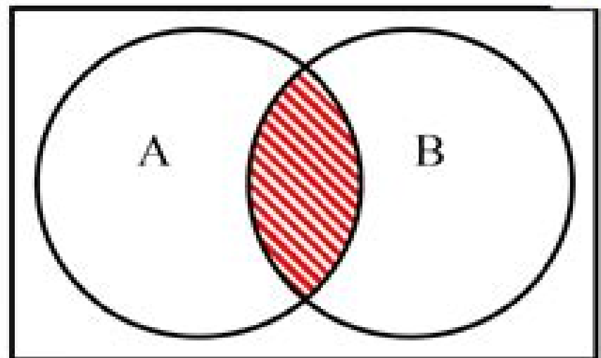
Set Intersection
