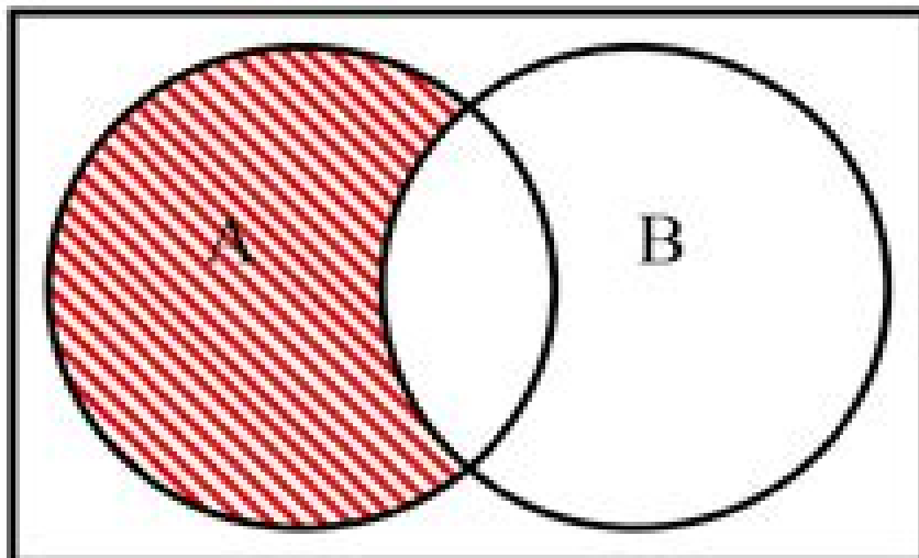
Set Difference
