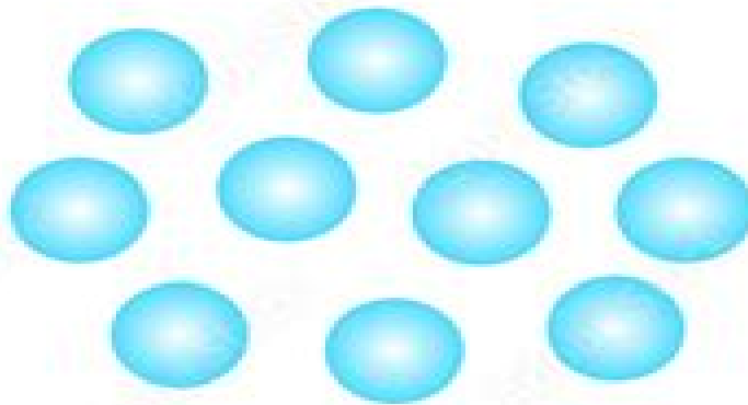
Monomers
