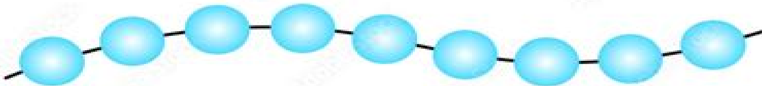
Polymer
