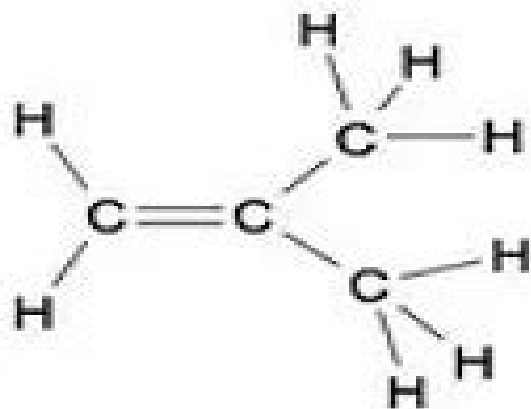
iso-butylene 2-methyl-propene (IUPAC name)
