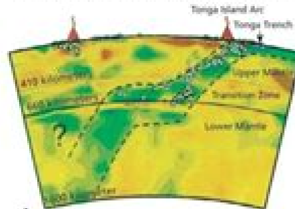
Seismic velocities Thermal mantle structure
