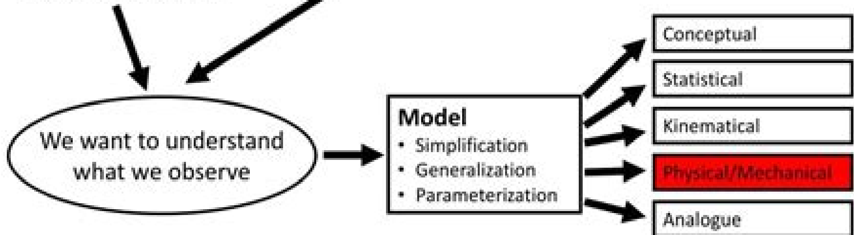
Folds, Boudinage, Reaction rims, Fractures
