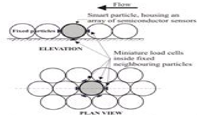
Figure 1: Test arrangement using the smart sediment particle
