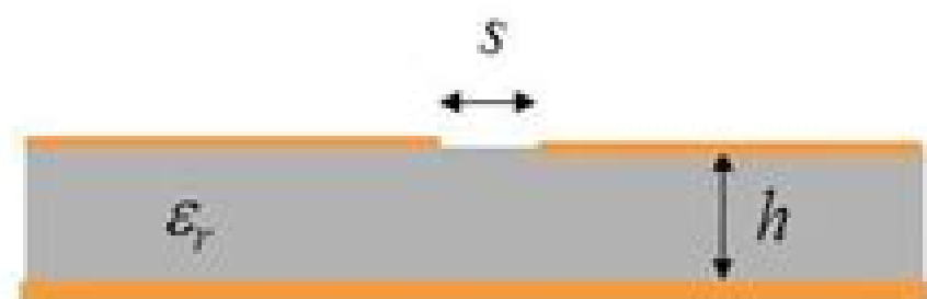
Conductor-backed Slotline
