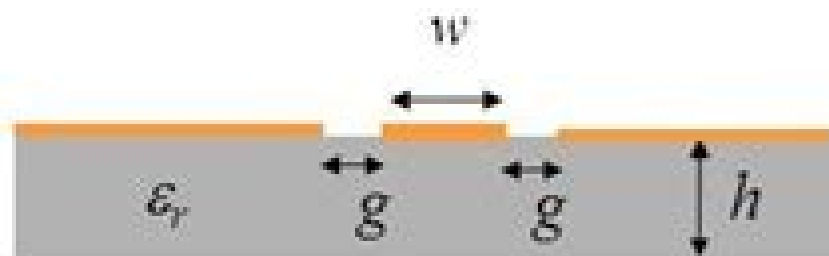
Coplanar Waveguide (CPW)
