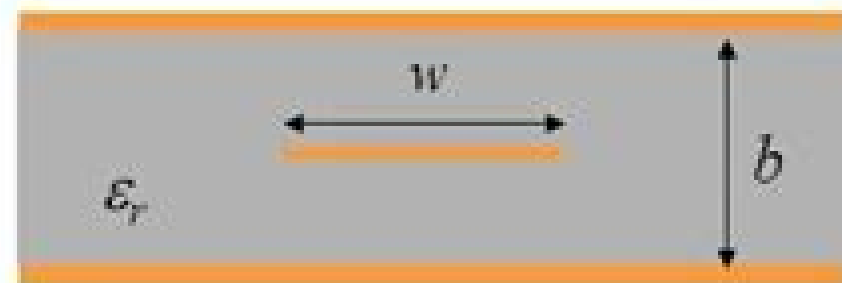
Stripline
