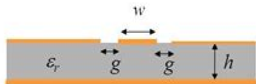
Conductor-backed CPW
