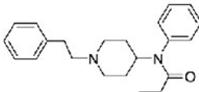
Fentanyl
