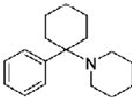
Phencyclidine (SN)
