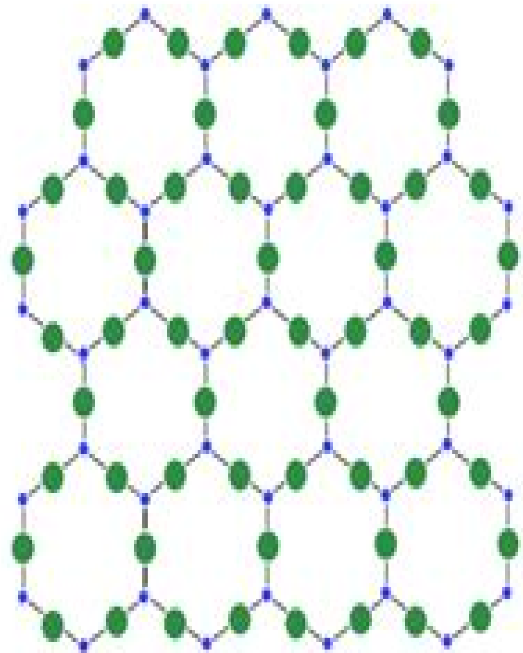
Crystalline Solids
