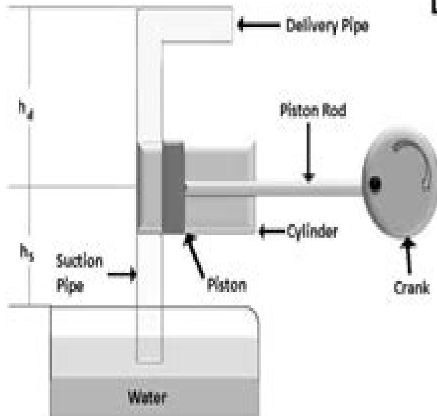
Reciprocating Pump
