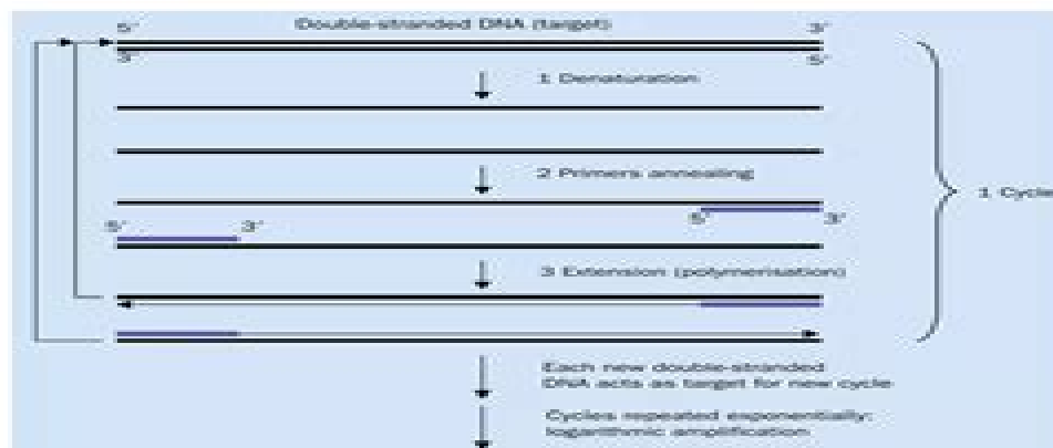
Figure 1. Schematic of PCR. The PCR reaction takes place in a thermocycler. Each PCR cycle consists of three major steps: (1) denaturation of template DNA into single-stranded DNA; (2) primers annealing to their complementary target sequences; and (3) extension of primers via DNA polymerisation to generate new copy of the target DNA. At the end of each cycle the newly synthesised DNA act as new targets for the next cycle. Subsequently, by repeating the cycle multiple times, logarithmic amplification of the target DNA occurs.
