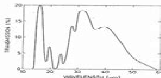
Fig. 2. Total transmission spectrum calculated for the combination consisting of 5 mm TPX, 1.2 mm polyethylene, and 3 mm KRS5 from Fig. 1.
