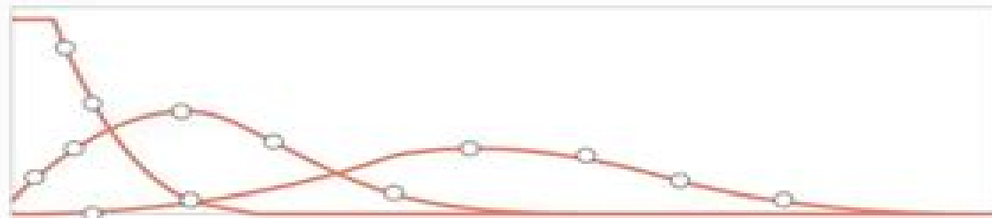
Poisson distribution
