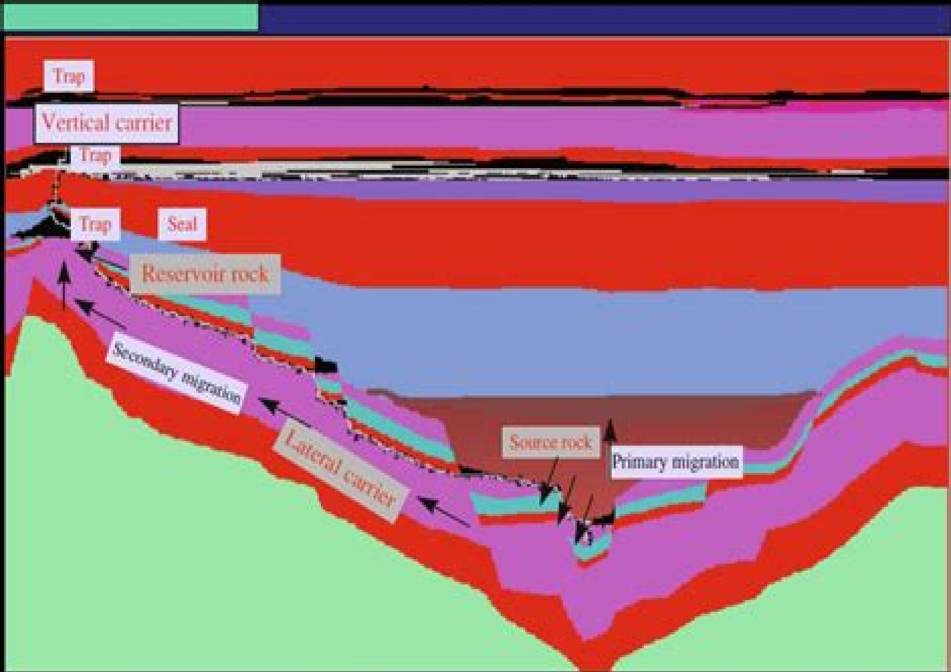
Petroleum migration
