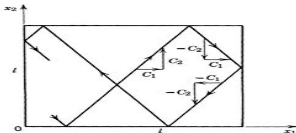
Fig. 2. Projection on the x_1, x_2 -plane of the path of a molecule in a cubical box in the fictitious situation of no intermolecular collisions and specular, elastic reflection at the walls.
