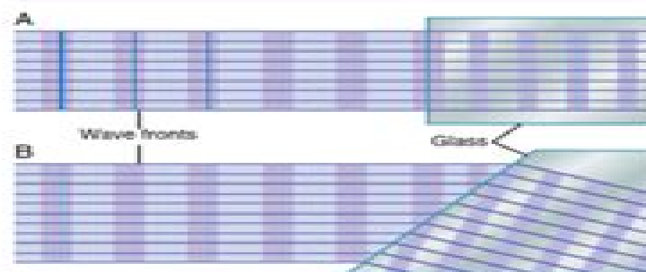
Figure 50-1. Light rays entering a glass surface perpendicular to the light rays (A) and a glass surface angulated to the light rays (B). This figure demonstrates that the distance between waves after they enter the glass is shortened to about two-thirds that in air. It also shows that light rays striking an angulated glass surface are bent.
