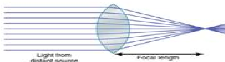
Figure 50-2. Bending of light rays at each surface of a convex spherical lens showing that parallel light rays are focused to a focal point.
