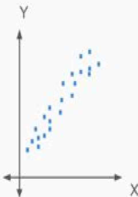
Positive Correlation
