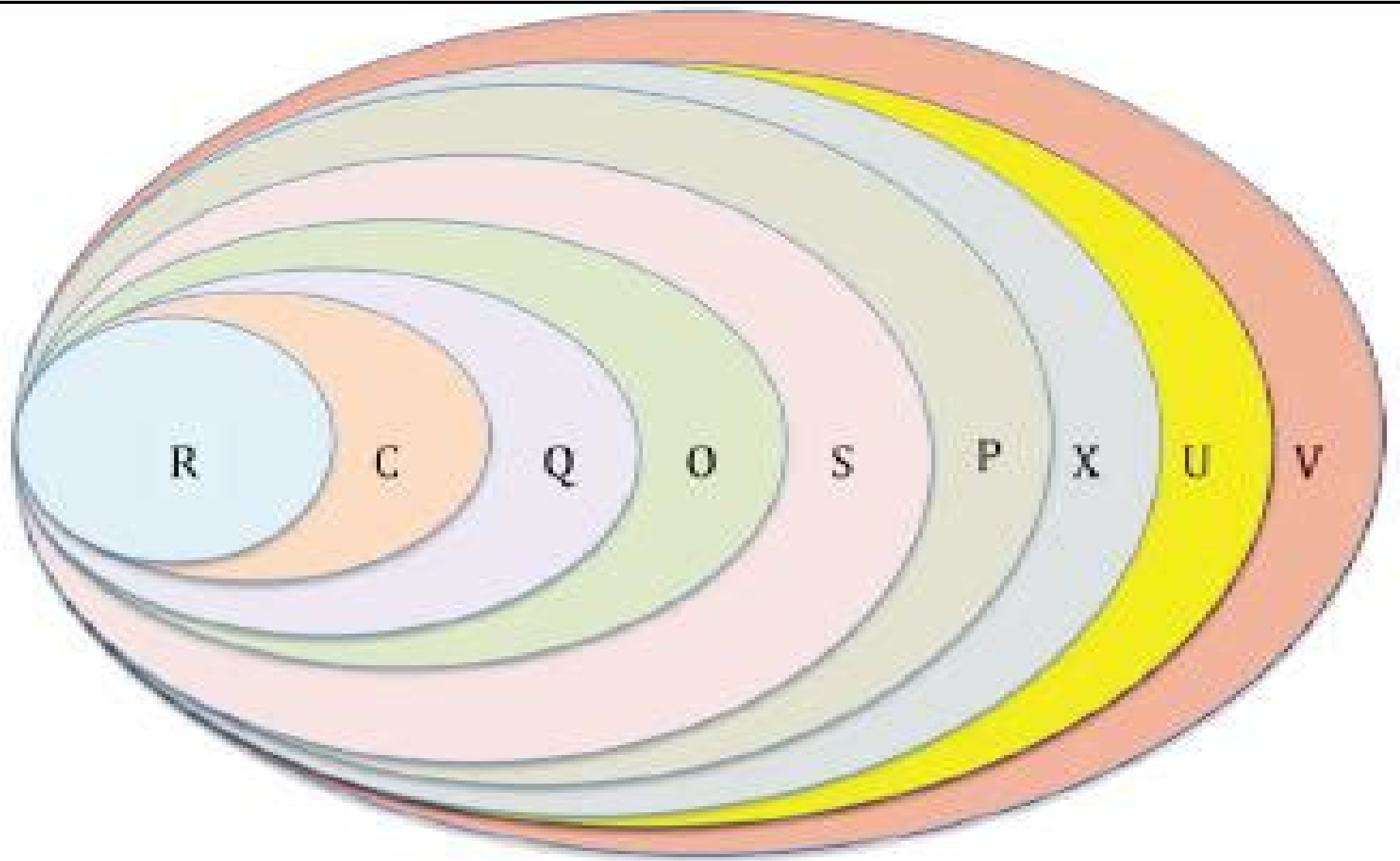
Figure 1: Enclosing sub-sets of the first nine Cayley-Dickson Hypercomplex Algebras. Reals (1D), Complex (2D), Quaternion (4D), Octonion (8D), Sedenion (16D), Pathion (32D), Chingon (64D), Routon (128D), and Voudon (256D).
